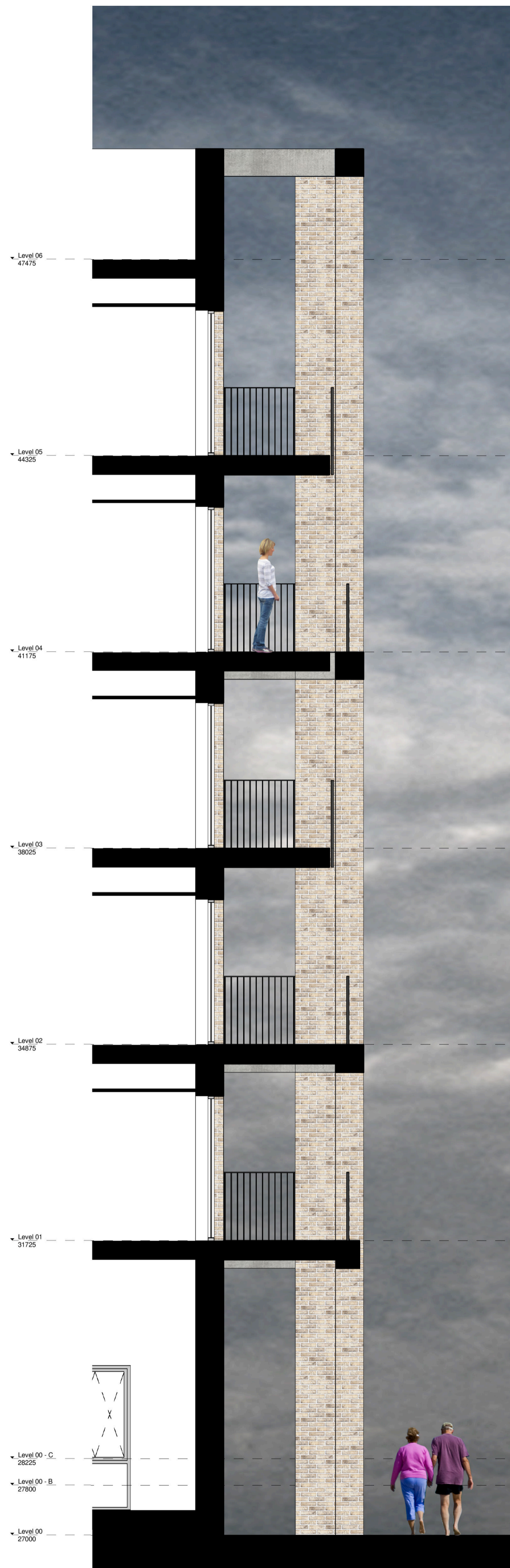
2 Block A Section Study 1:50
